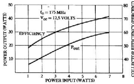
POWER OUT AND EFFICIENCY vs POWER IN
